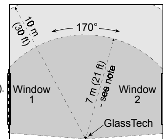
Figure 1. Coverage Pattern
